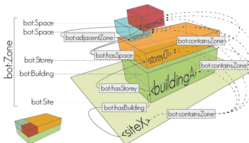
Figure 9: BOT allows representing the topology of a building: Site, Building, Storey, Space, Element, Interface. 33
