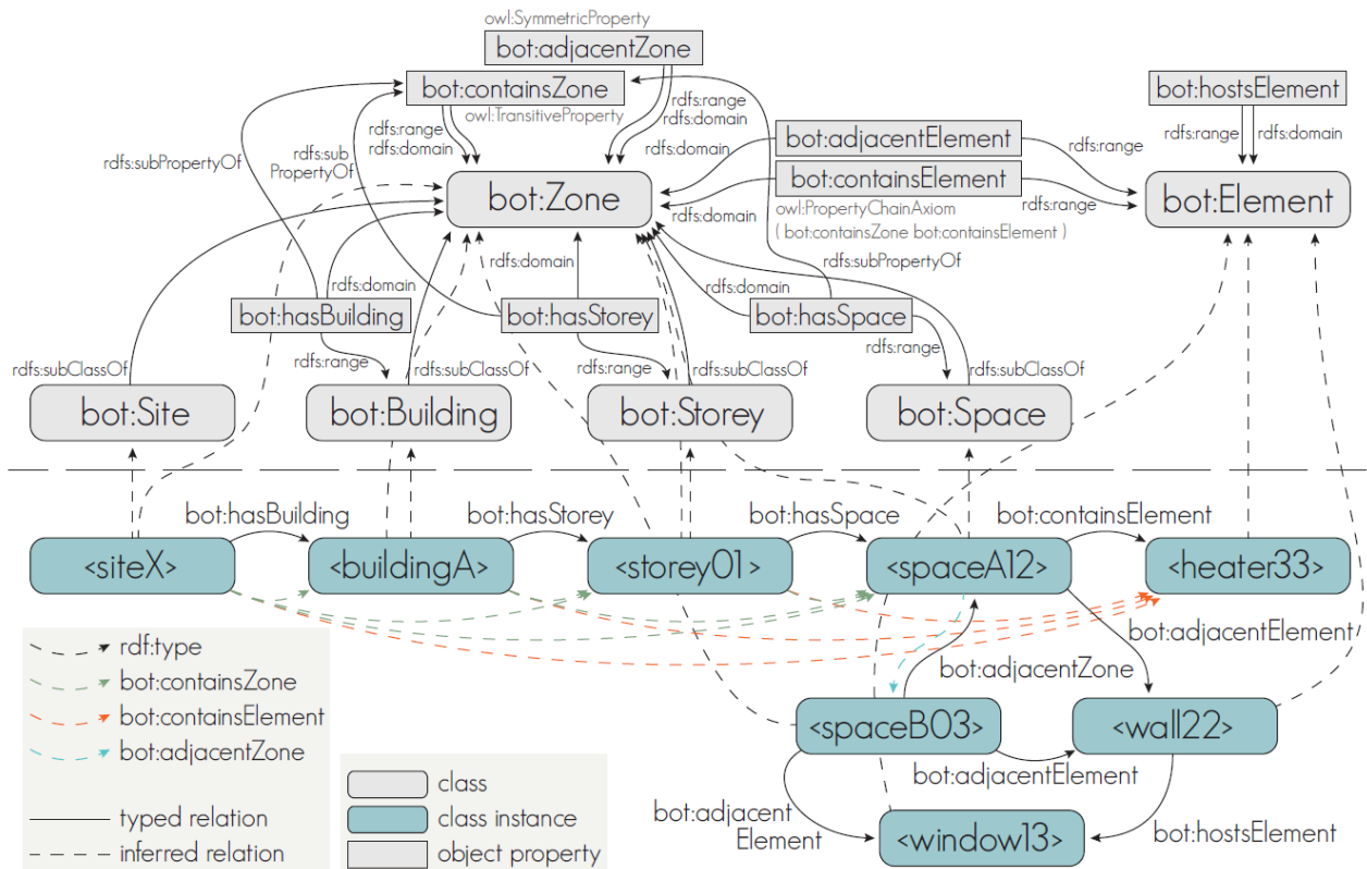
Figure 10: Example use of BOT for an example building 34 .
